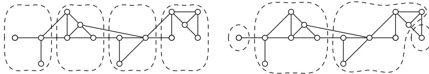
Figure 1: Two P_4 -witness structures of a graph.
