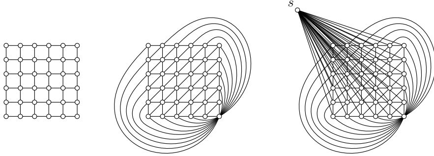
Figure 2: The graphs M_6 , \Gamma_6 , and \Pi_6 , respectively.
