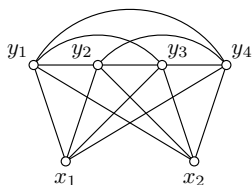
Figure 3: The graph H_4^*(2) .
